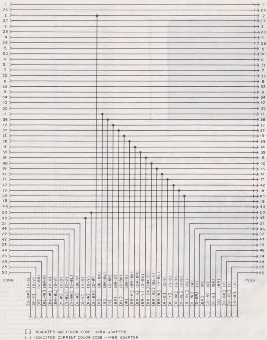
Fig. 2—148A (MD) and 148B Adapter, Schematic
