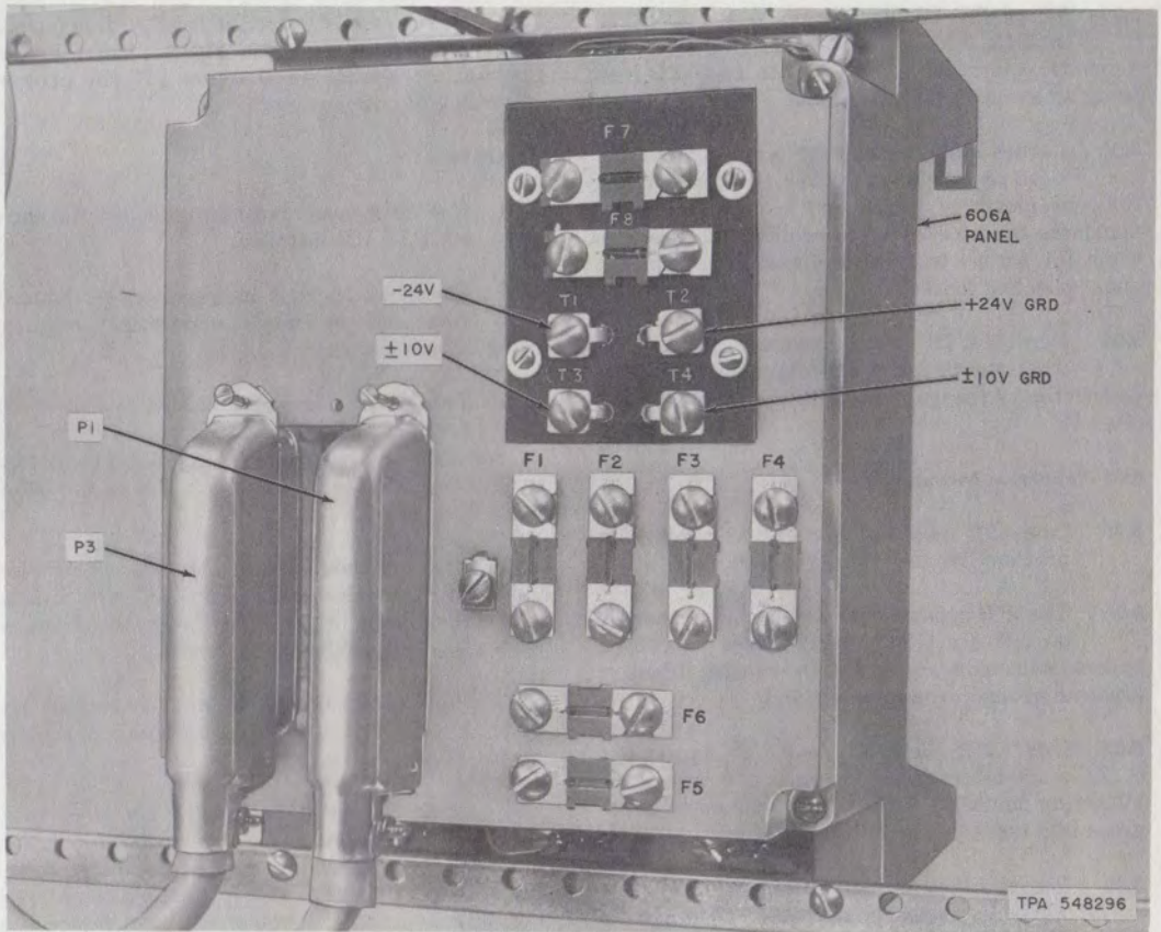
◆ Fig. 4—606A Panel (Rear View) ◆
