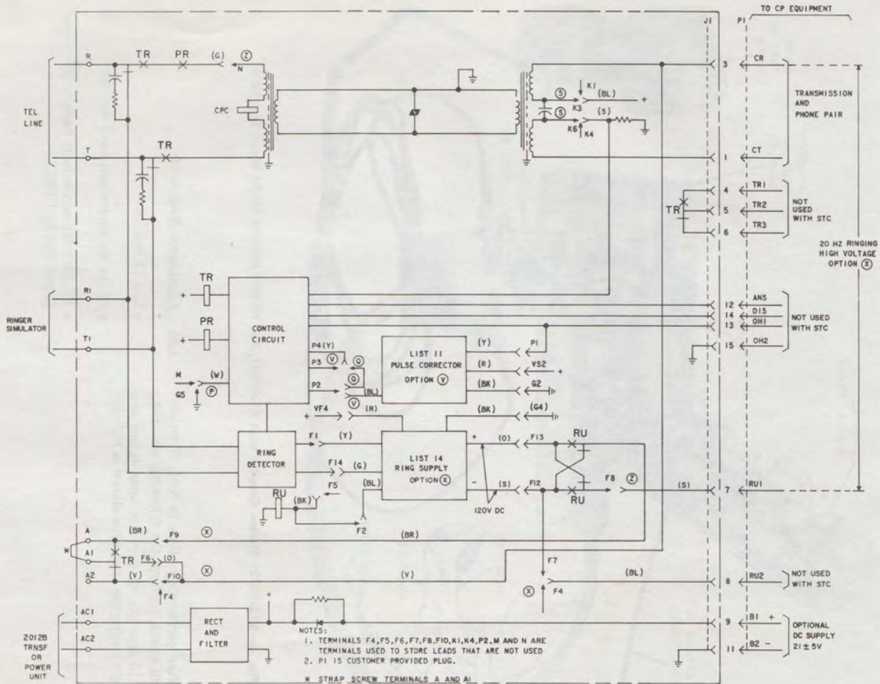
Fig. 7—KS-20721 Station Coupler Internal Wiring Options
