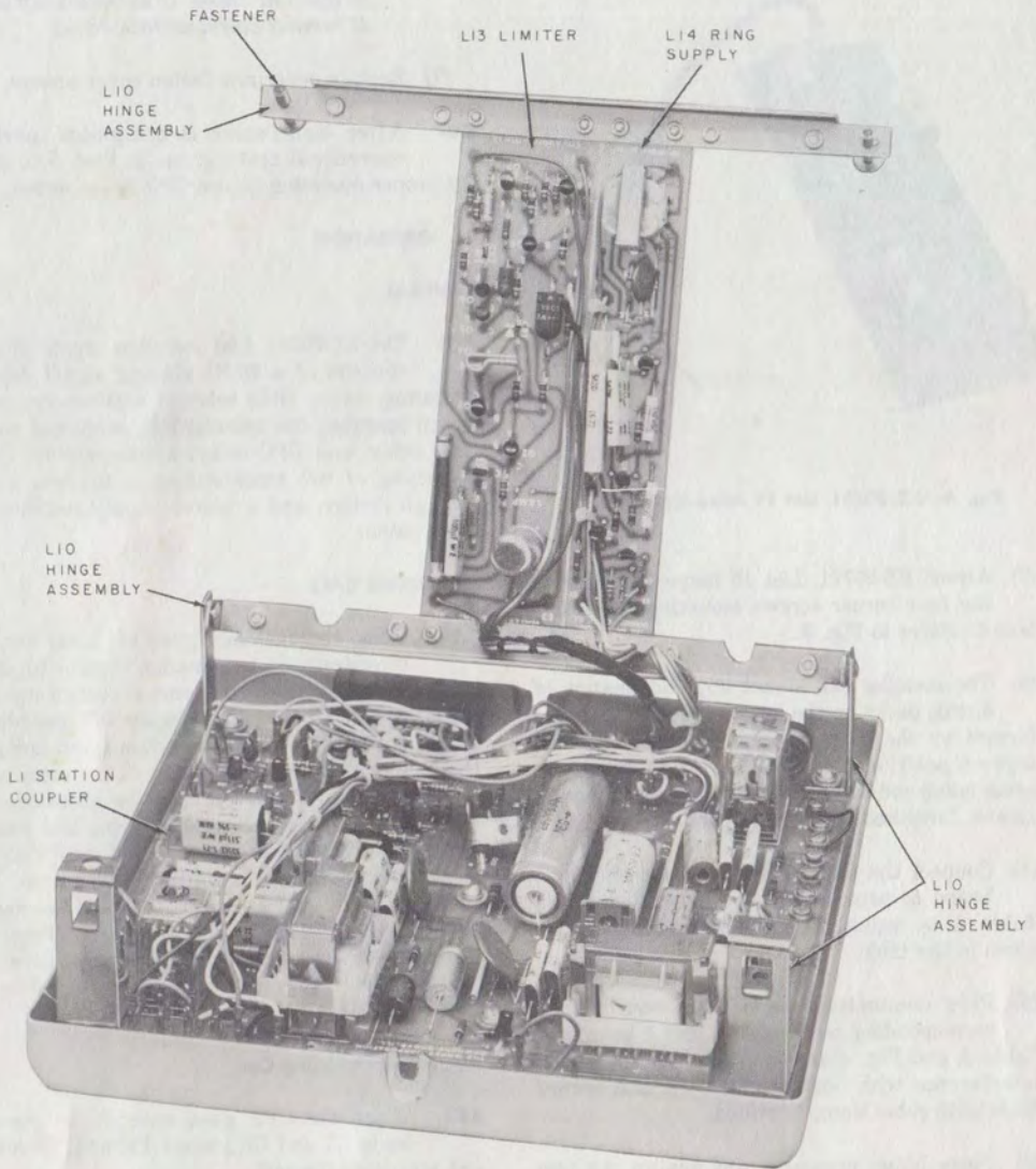
Fig. 3—KS-20721 Station Coupler Showing Optional Circuit Packs
