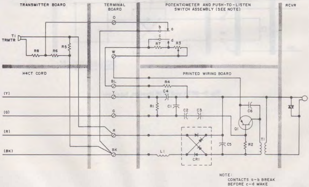
Fig. 8—G8B Handset, Schematic
