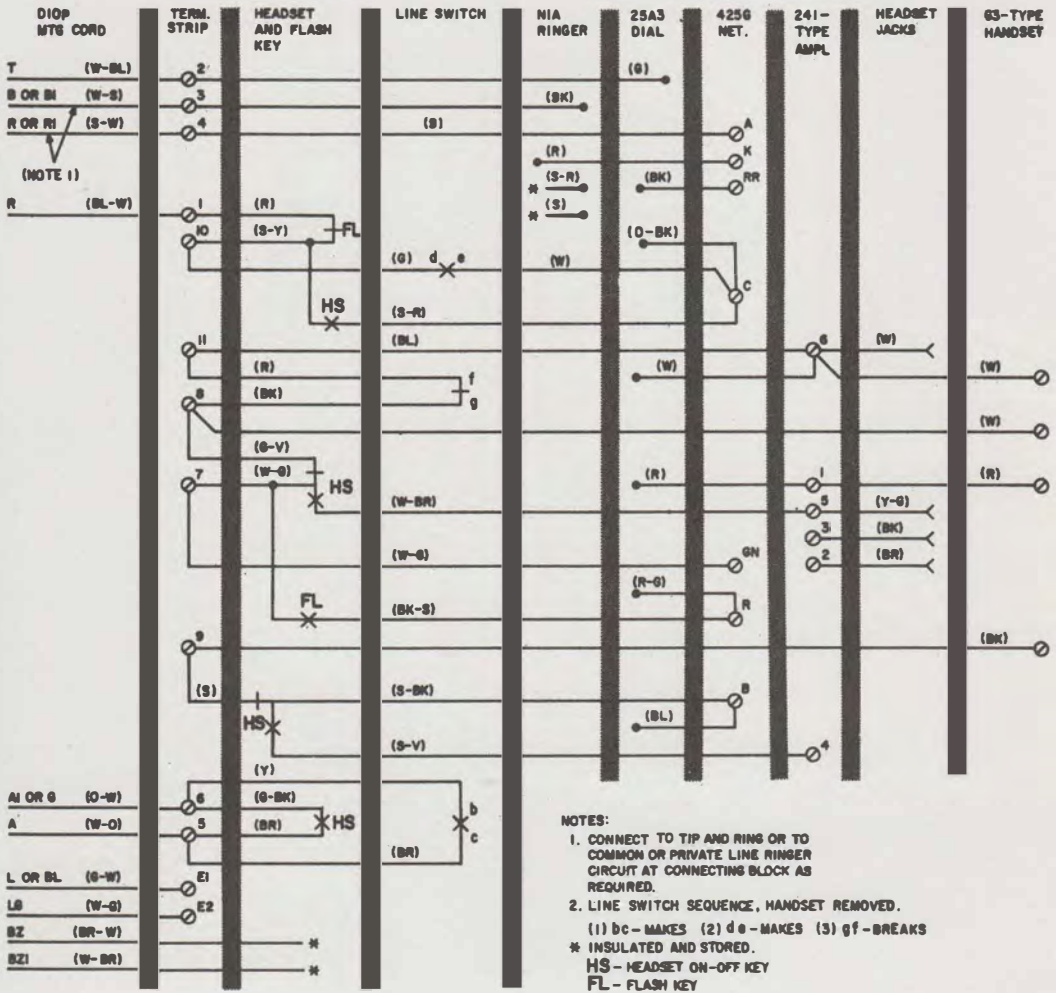
Fig. 2—1514B (MD) Telephone Set Connections With 25A3 (MD) Dial (Early Production)
