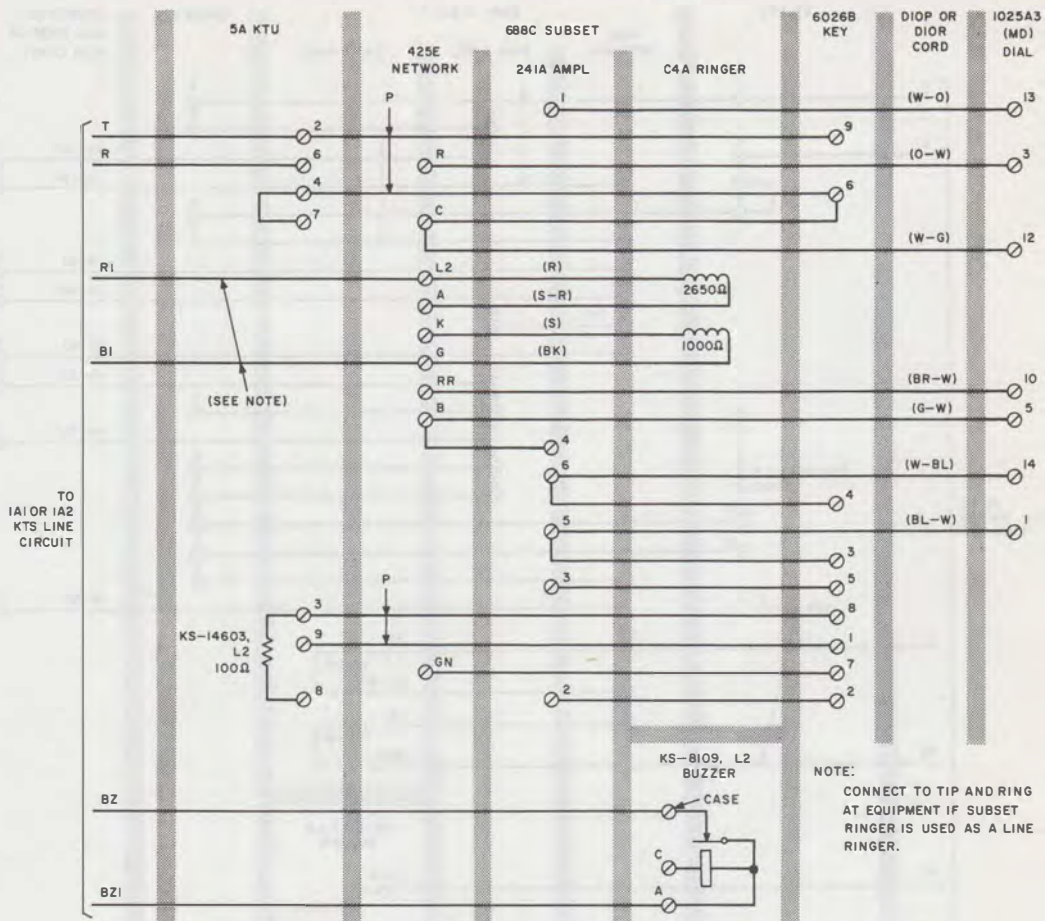
Fig. 10—688C Subset and 1025A3 (MD) Dial, With Hold
