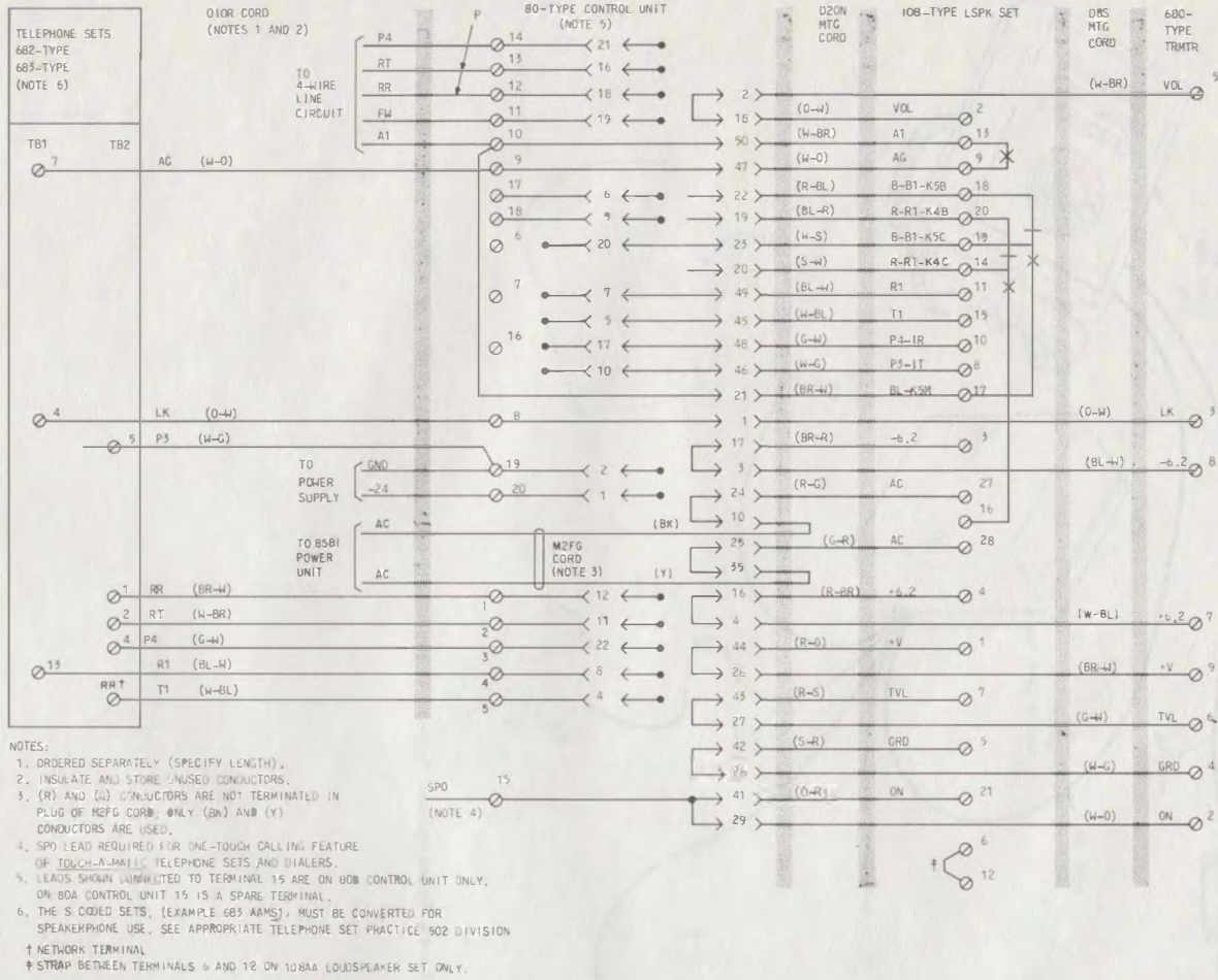
Fig. 2—4A Speakerphone Connections, Telephone Set Equipped With a Rotary Dial
