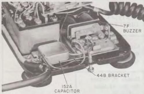
Fig. 13—7F Buzzer and 152A Capacitor Mounted on 44B Bracket
