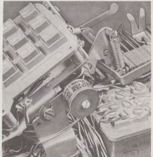
Fig. 9—KS-20419L1 Buzzer Mounted on TOUCH-TONE® Dial Mounting Screw
