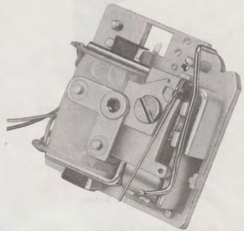
Fig. 3—9A Buzzer With Cover (64A Gong) Removed
