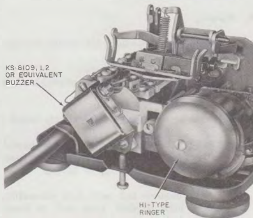
Fig. 11—KS-8109 Type Buzzer Mounted on Bracket of H1A Ringer
