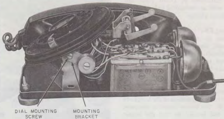
Fig. 8—KS-20419L1 Buzzer Mounted in 500-Type Telephone Set
