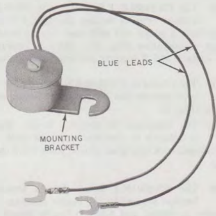
Fig. 7—KS-20419L1 Buzzer
