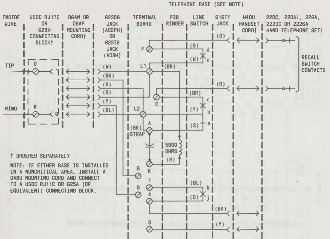
Fig. 11—AC2PH or AD3H Telephone Base Connections With 220C, 220AL, 226A, 2220C, or 2226A Hand Telephone Set
