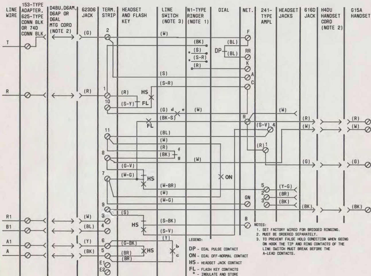
Fig. 2—514BM Telephone Set, Connections
