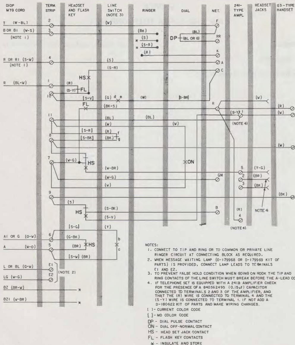
Fig. 1—514B Telephone Set, Connections
