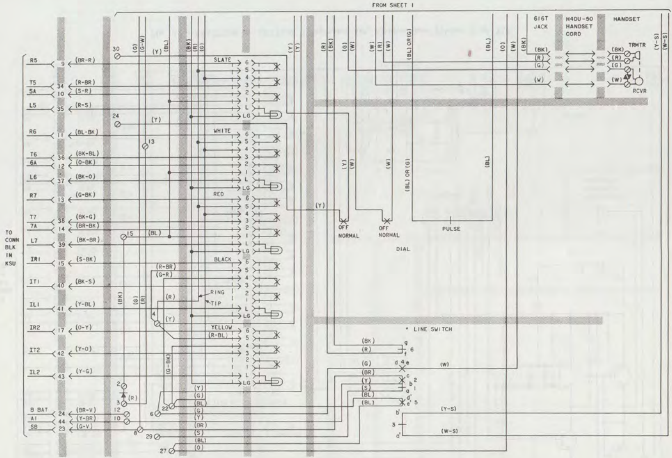
Fig. 10—832BM or 832DM Telephone Set, Connections (Sheet 2 of 2)
