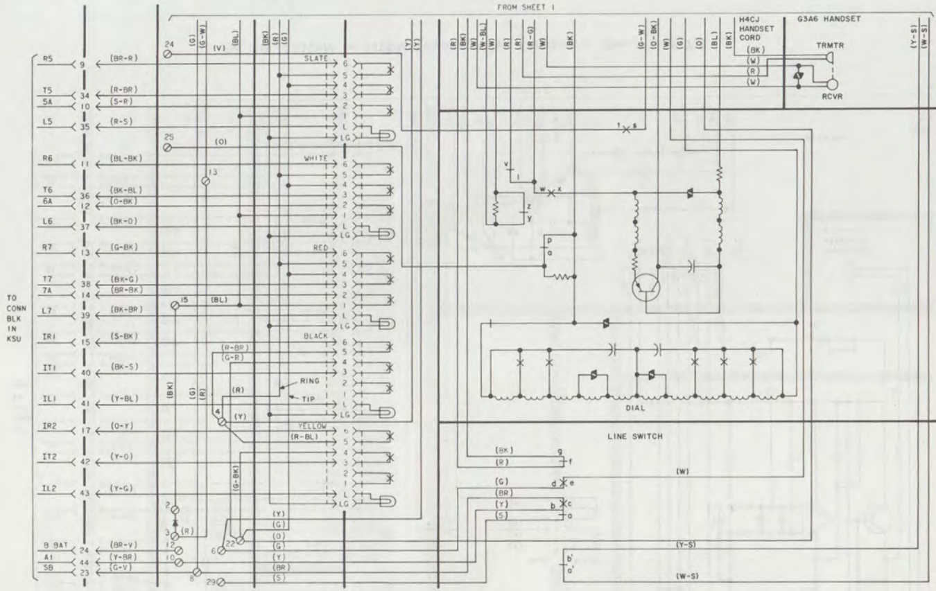
Fig. 9—2832B (MD) Telephone Set, Connections (Sheet 2 of 2)
