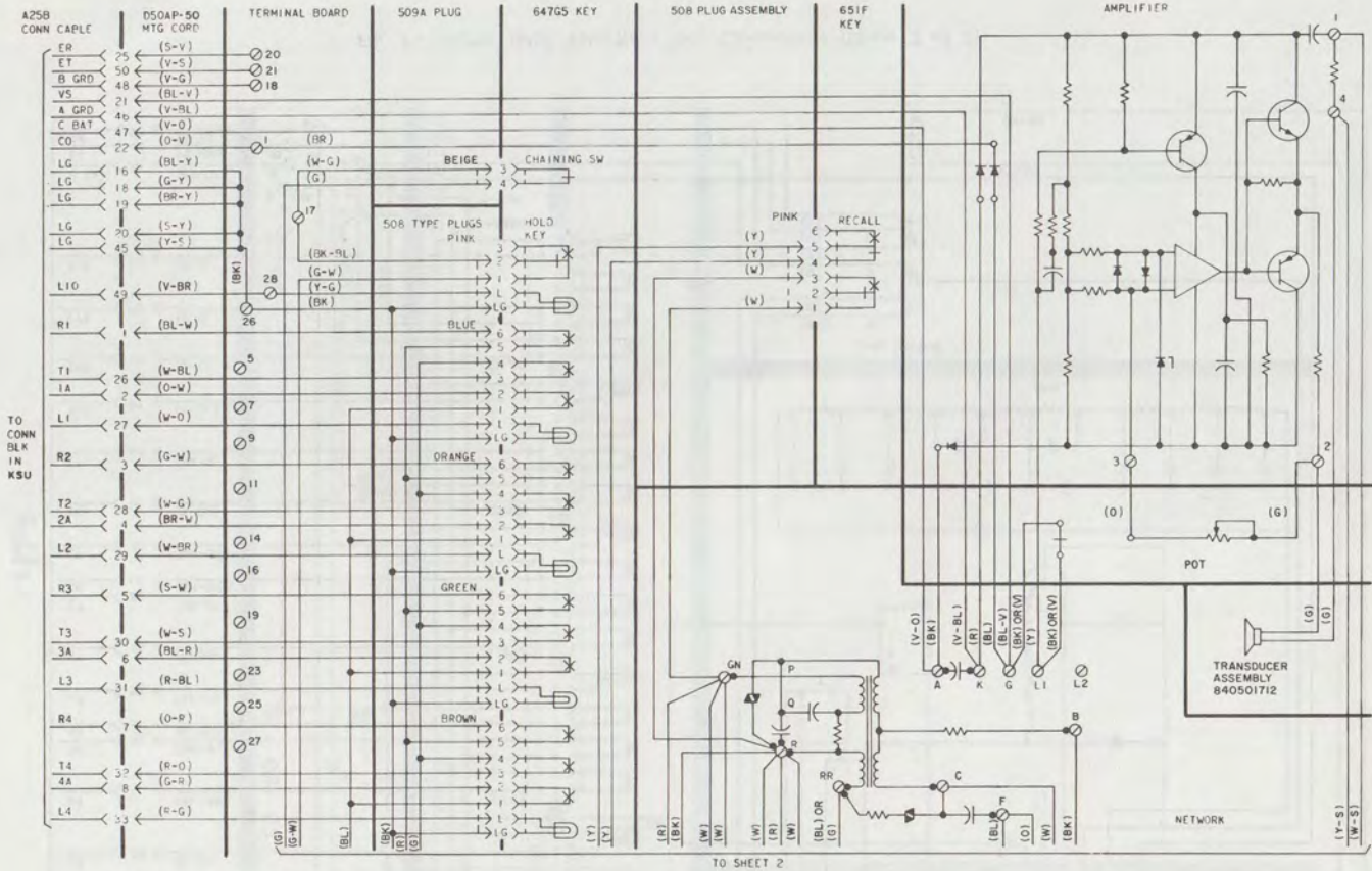
Fig. 8—832B (MD) Telephone Set, Connections (Sheet 1 of 2)
