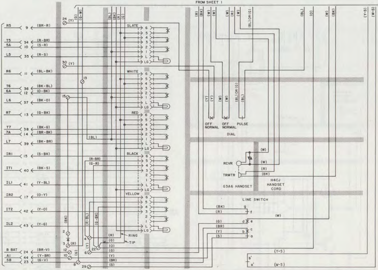
Fig. 6—832A (MD) Telephone Set, Connections (Sheet 2 of 2)
