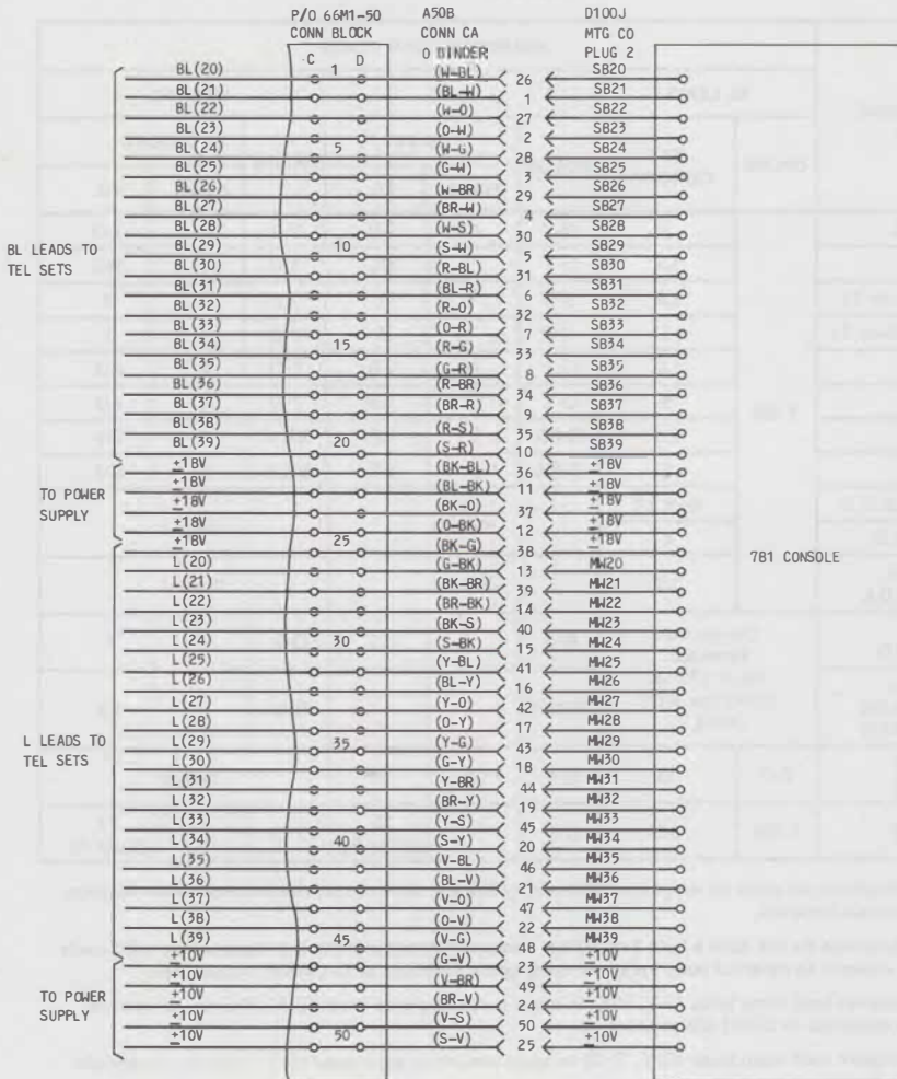
Fig. 3—7B1 Console Connections (Sheet 2 of 2)
