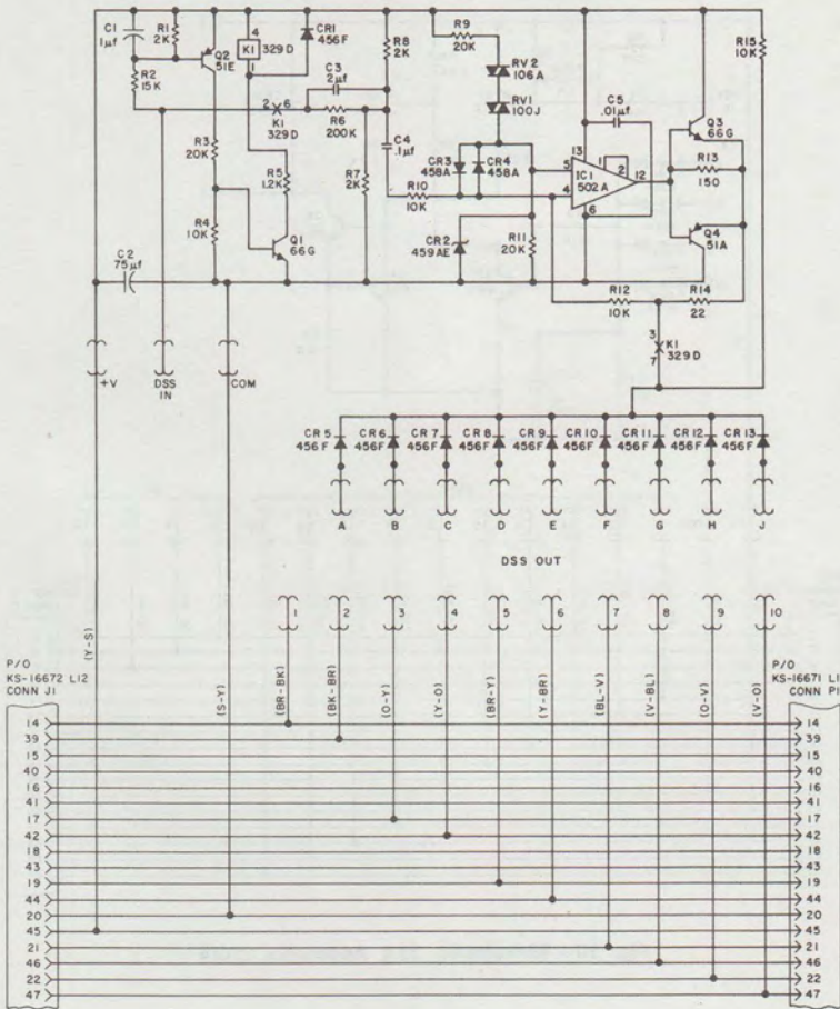
Fig. 31—Schematic, 26A Apparatus Unit
