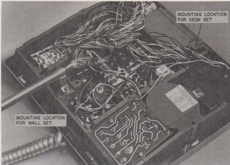
Fig. 8—Set Modification For Wall Mounting
